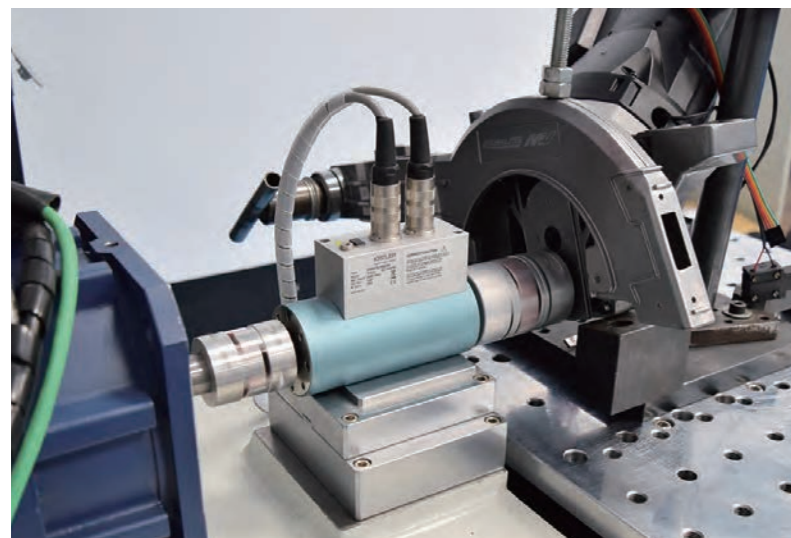
Brushless DC Motor test for Characteristics
